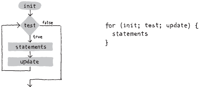
Figure 4-1. Flow diagram of a for loop.
